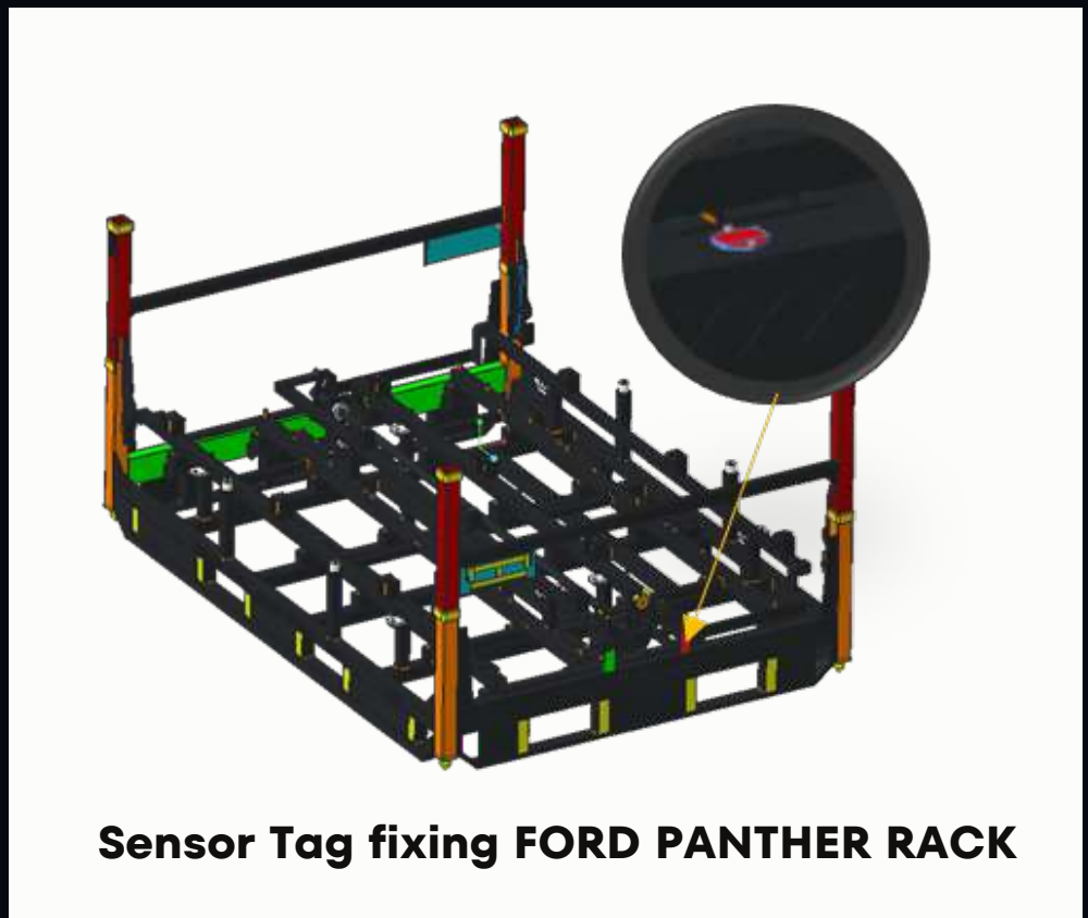
BLE Signal Transmitting Sensor Tag (A Product of BOSCH)
